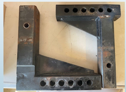
2" & 2 1/2" Hitch Shank
