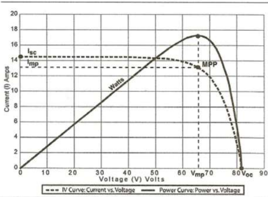
Figure 5. MPPT Optimum Power Point Charging
